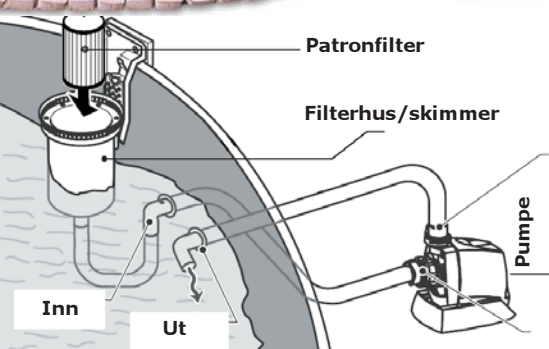
Splasher Pool med patronfilter. (Atlantic Pools)
