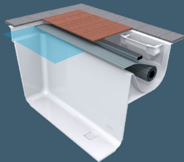
The roller shutter shaft extends the pool by 80 cm.
