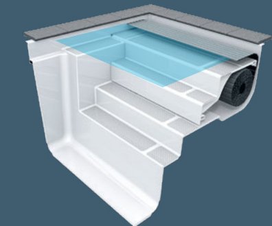
The roller shutter shaft extends the pool by 25 cm.
