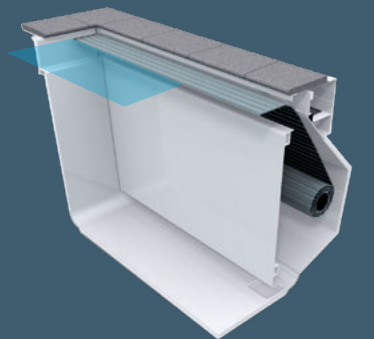
The niche extends the pool by approx. 35 cm and shortens the swimming length by approx. 50 cm.
