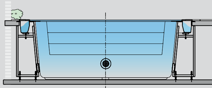
Self-supporting installation with laminated steel wall supports (pool with overflow channel)
