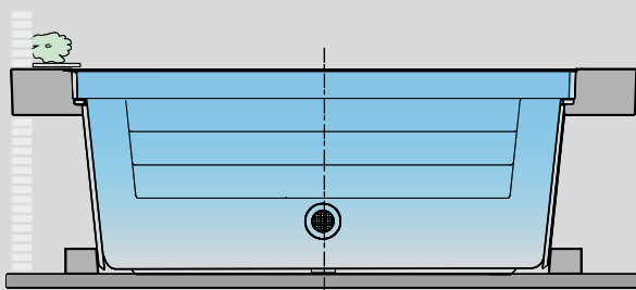
Self-supporting installation with laminated steel wall supports
