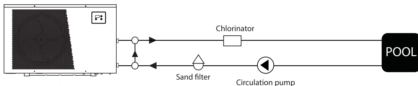
Outline diagram for installation of X-series
