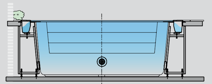
Self-supporting installation with laminated steel wall supports (pool with overflow channel)
