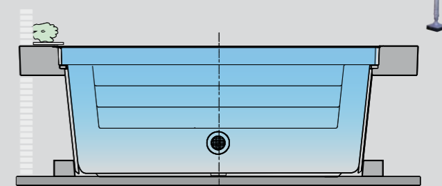
Self-supporting installation with laminated steel wall supports
