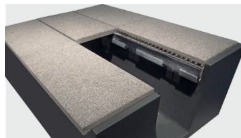
Overflow channel with stone cover adjustable overflow weir of V4A
