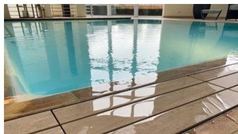
Overflow channel with stone cover adjustable overflow weir of GRP
