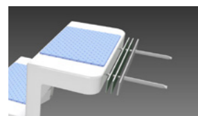
Fixation with wall anchors V4A for for Eleganz 60 + 80 K (short version)
