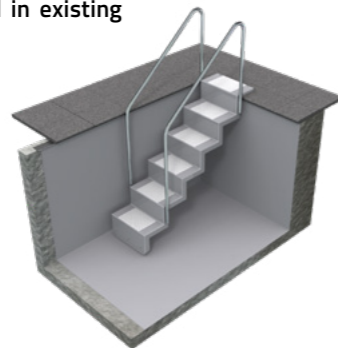
5 steps, long version, fixed with 2 bolts in the coping stone. Rubber base plate on the floor without fixings.
