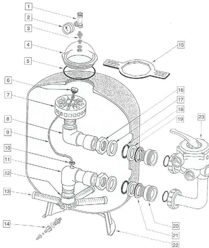
Triton™ (old version) Sand Filter
